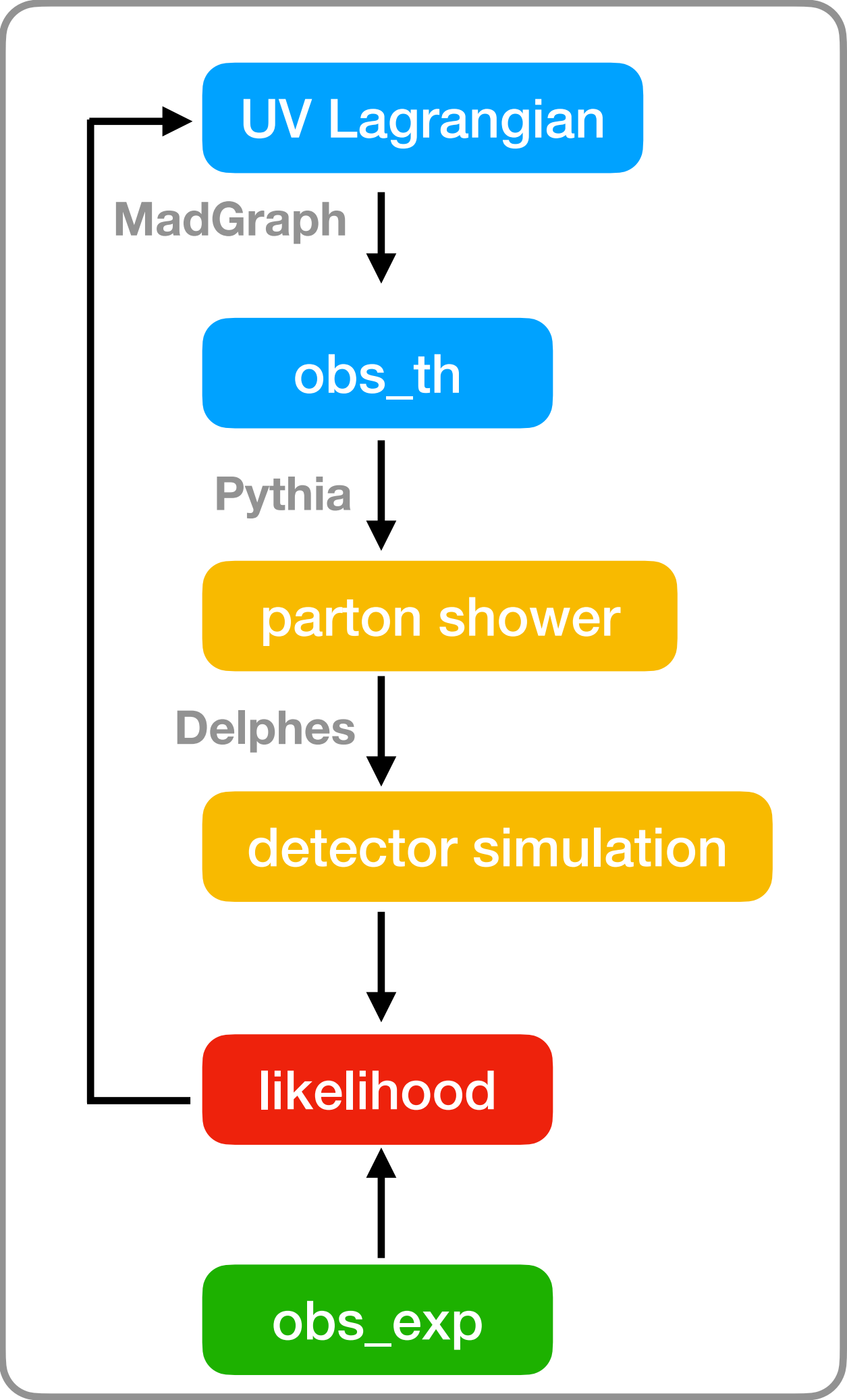
workflow of collider study
