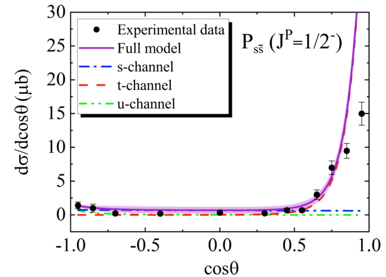
FIG. 9. The differential cross section d\sigma/d\cos\theta for the \pi^- p \rightarrow K^* \Sigma reaction as a function of \cos\theta . The experimental data are from Ref. [35]. Here, the notation is the same as that in Fig. 8.
